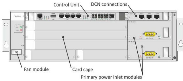
Fig 1. TM-301/II Chassis.
